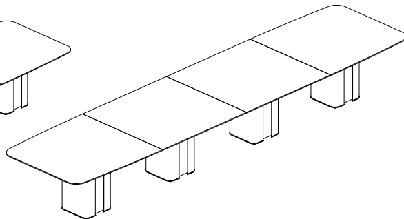
MT7 | L*W*H 420 120 75 420 140 75
