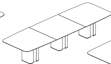
MT6 | L*W*H 280 120 75 280 140 75
