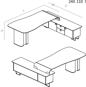
7 | L*W*H*D 240 110 75 200
