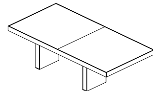
MT3 L * W * H 211.6 101.6 75 241.6 121.6 75
